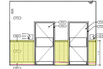
7 RESTROOM HALL ELEVATION
