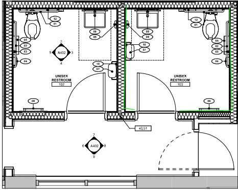
1 ENLARGED RESTROOM PLAN
