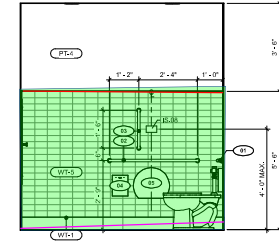
5 TYPICAL RESTROOM ELEVATION
