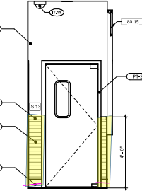
8 RESTROOM HALL ELEVATION
