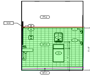
3 TYPICAL RESTROOM ELEVATION
