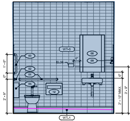
2 TYPICAL RESTROOM ELEVATION
