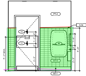
4 TYPICAL RESTROOM ELEVATION
